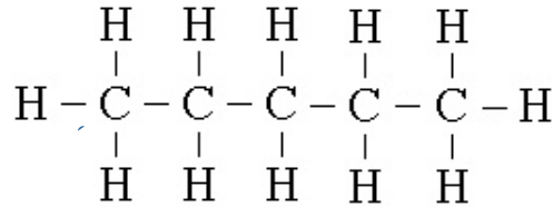
pentano (C 5 H 12 )
